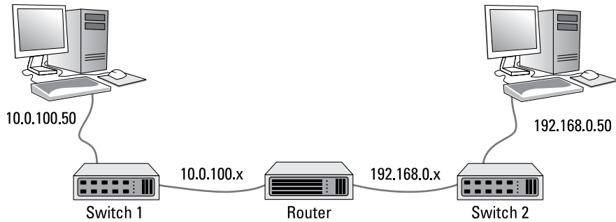
FIGURE 3-3: Two IP networks connected by a router.
