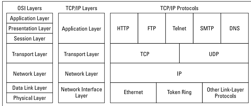
FIGURE 1-7: TCP/IP and the OSI model.
