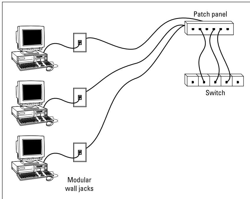
FIGURE 1-2: Using wall jacks and patch panels.
