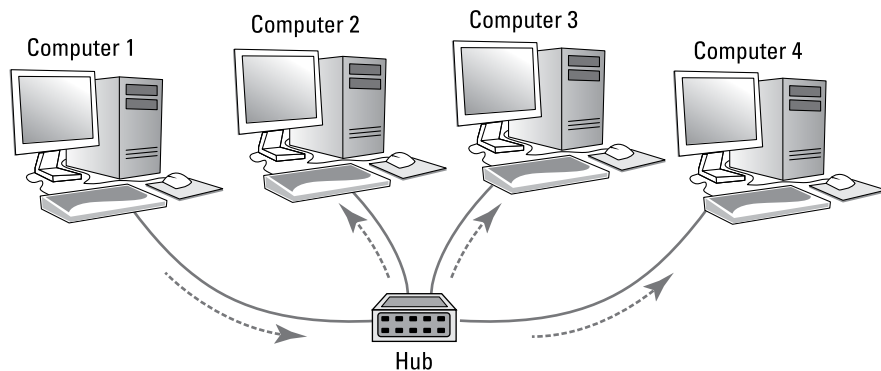
FIGURE 3-1: A hub repeats all incoming data on all its ports.
