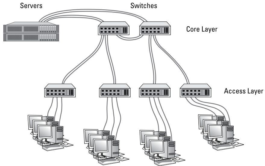
FIGURE 1-7: A two-tiered switch design.
